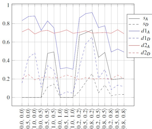
Figure 2: Comparison of performance between static and adaptive autonomy [6].
