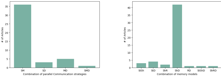
(a) Combination of communication models. S - Shared memory, M - Message passing, D - Data flow (b) Combination of memory models. St - Stack based, Sh - Shared, R - Region based, D - Distributed
