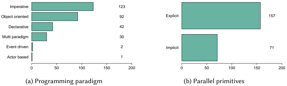
Fig. 6. Language properties: programming paradigm and parallel primitives
