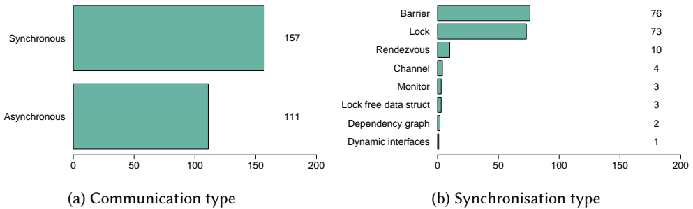
Fig. 8. Language properties: communication and synchronisation types
