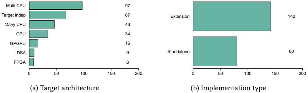
Fig. 14. Target architecture and implementation type
