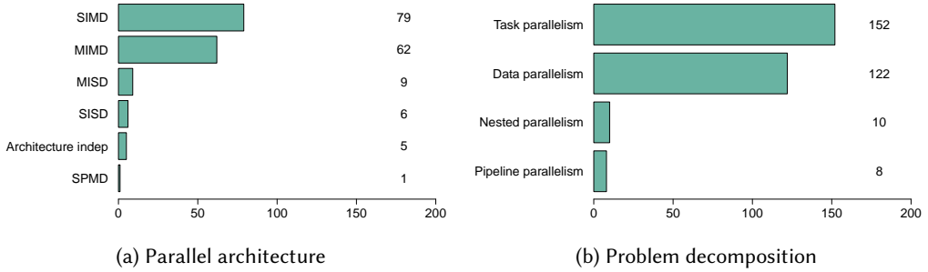
Fig. 9. Programming model: parallel architecture and problem decomposition
