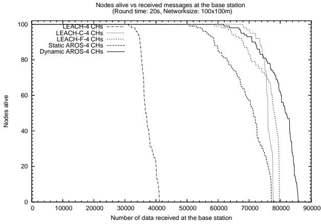
Figure 7. Simulation results from the simulations in a 100x100 meter network
